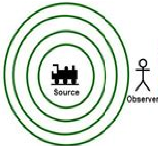
Source & Observer at Rest
