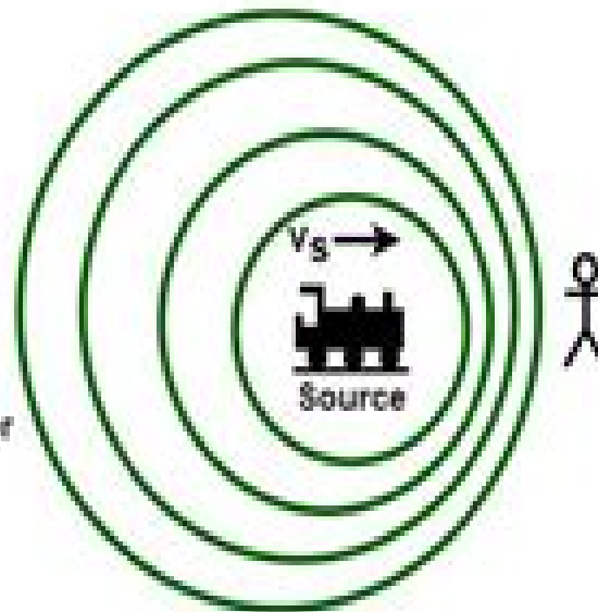
When the Source is moving toward Observer at Rest
