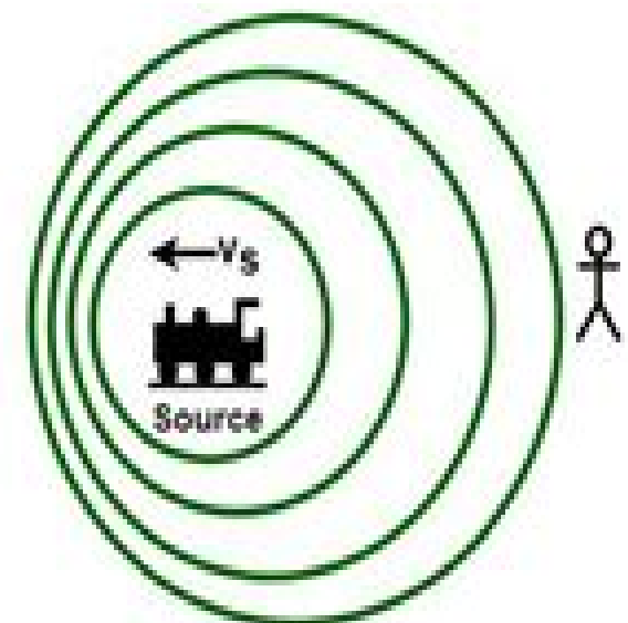
When Source is moving away from Observer at Rest
