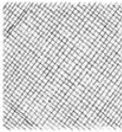
Cross- Hatching
