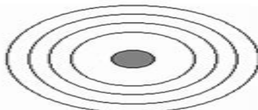
Chlorine
