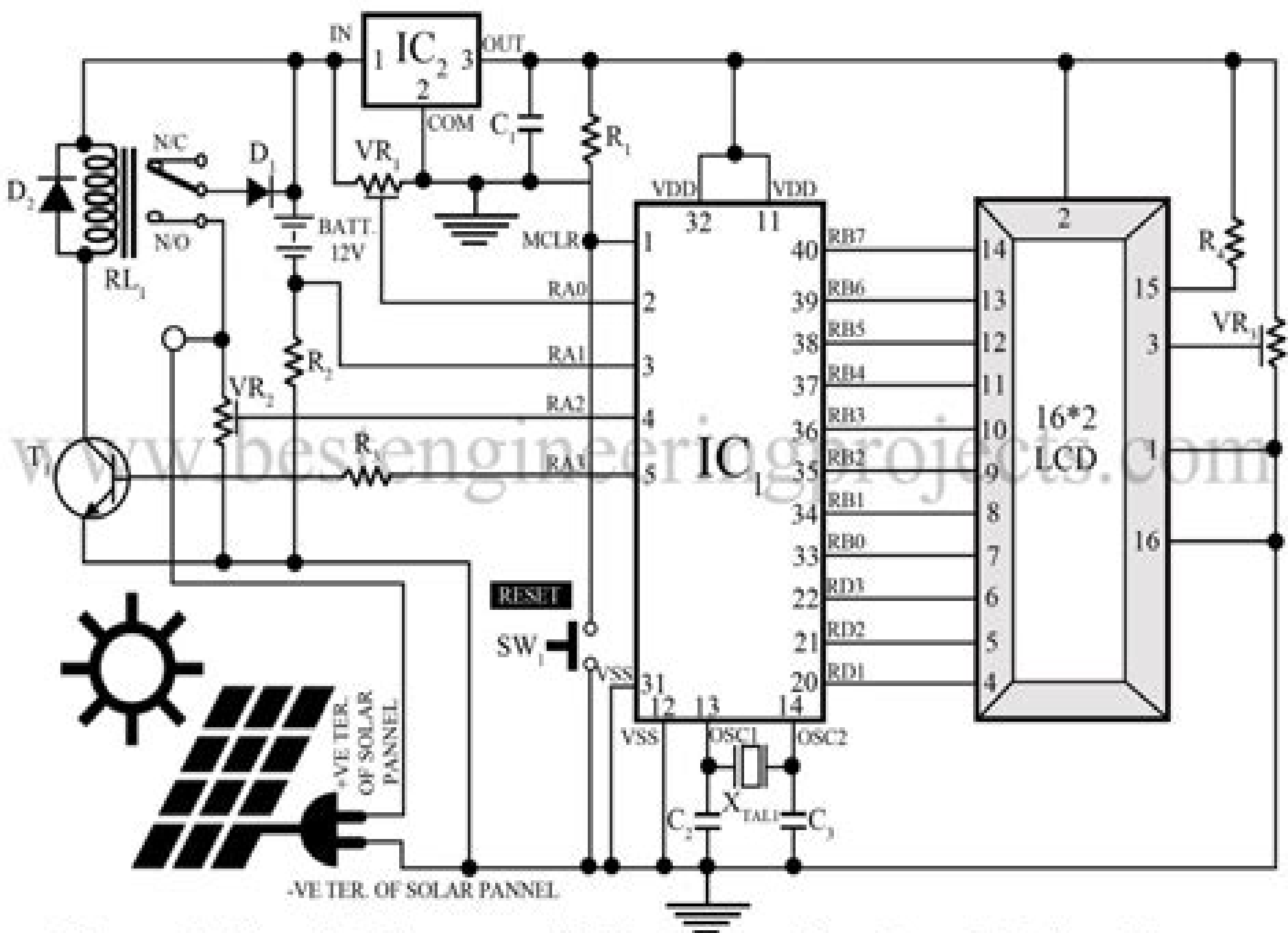
Figure 1 Circuit Diagram of Microcontroller Based Solar Charger
