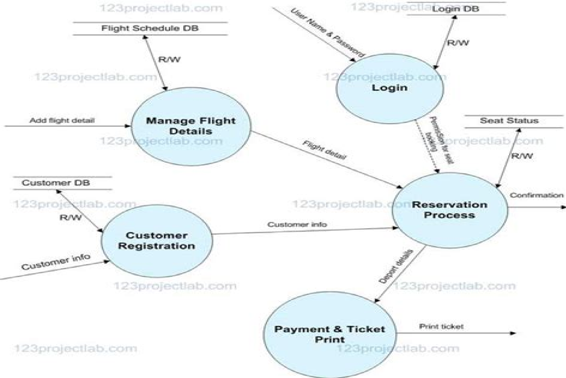
Level 1 DFD for Airlines Reservation System
