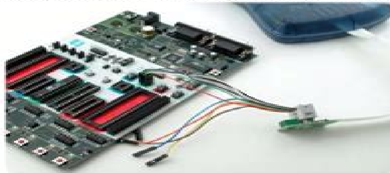
Figure 2. Connecting JTAGICE mkII probe to 6-pin ISP header using the squid cable
