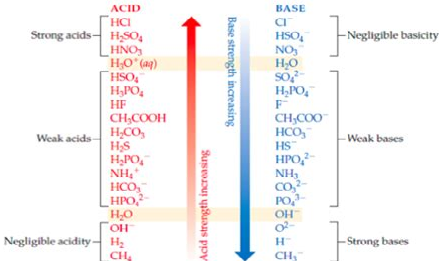
▲ FIGURE 16.3 Relative strengths of select conjugate acid–base pairs. The two members of each pair are listed opposite each other in the two columns.
