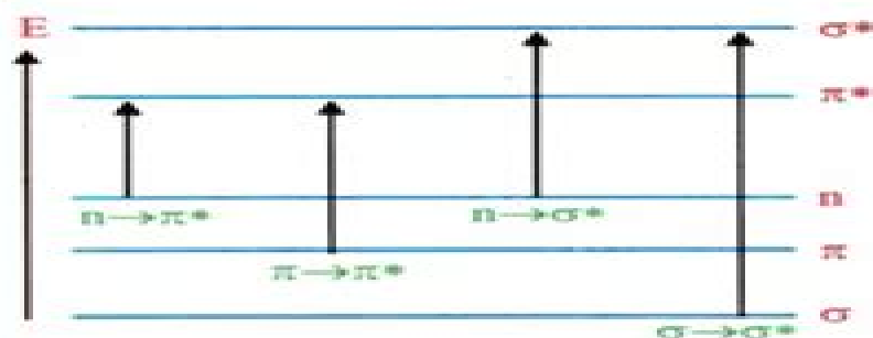
Fig 13.5: Electron transition in organic compound due to interaction with U.V-visible radiations
