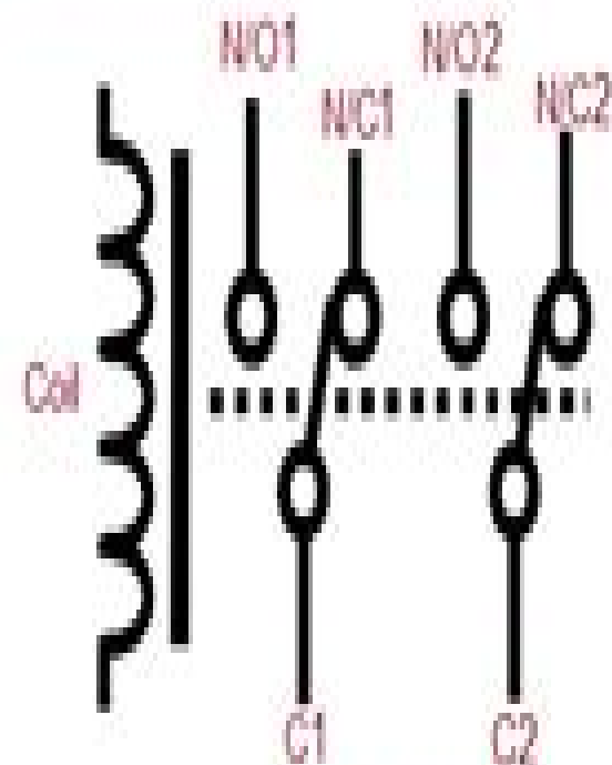
DPDT Symbol
