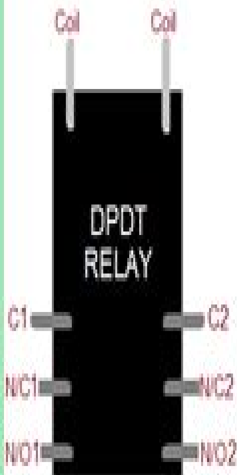
bottom view
