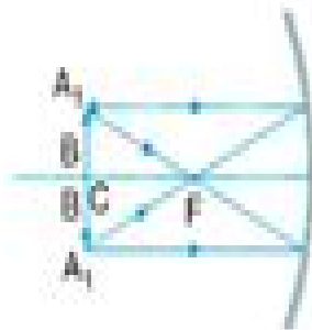
Real, inverted image of the same size as object at C
