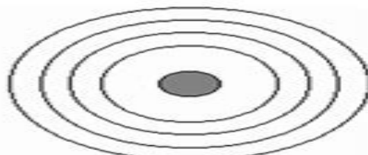
Chlorine
