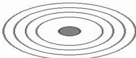
Neon
