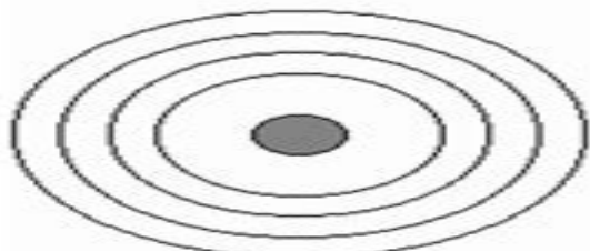
Magnesium
