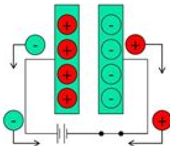
Charged Capacitor
