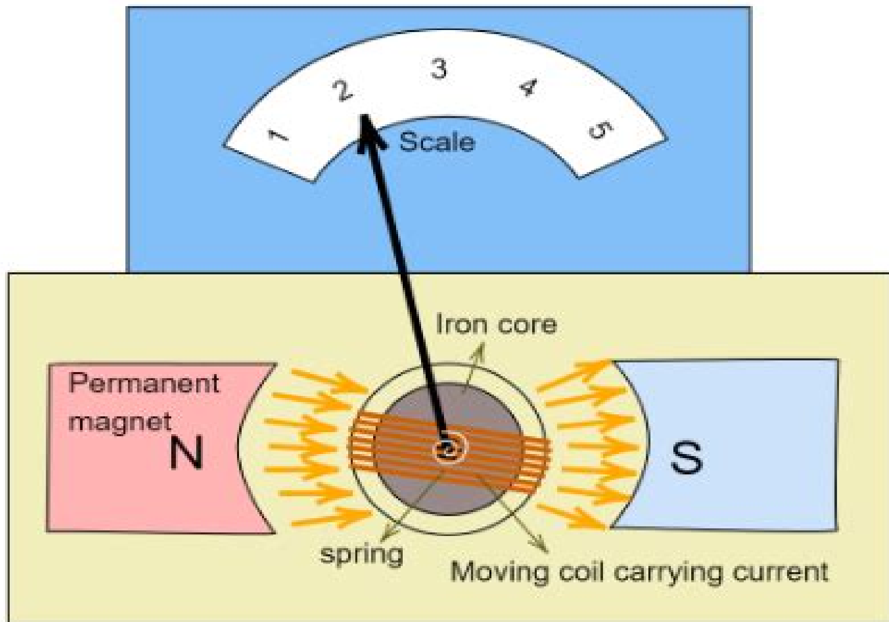
Front view of a Moving Coil Galvanometer
