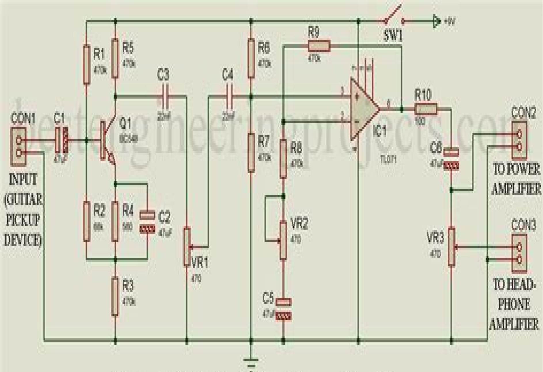
Figure 1: Electric Guitar Preamp Circuit
