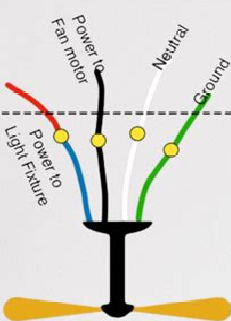
Red wire from ceiling connecting Blue wire from fan
