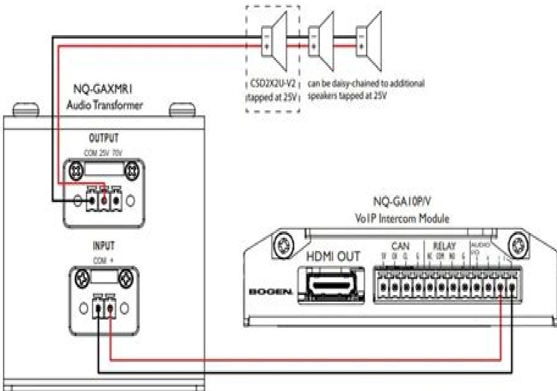
Figure 7: NQ-GA10P/V VoIP Intercom Module connected to NQ-GAXMR1 Audio Transformer then to speaker.
