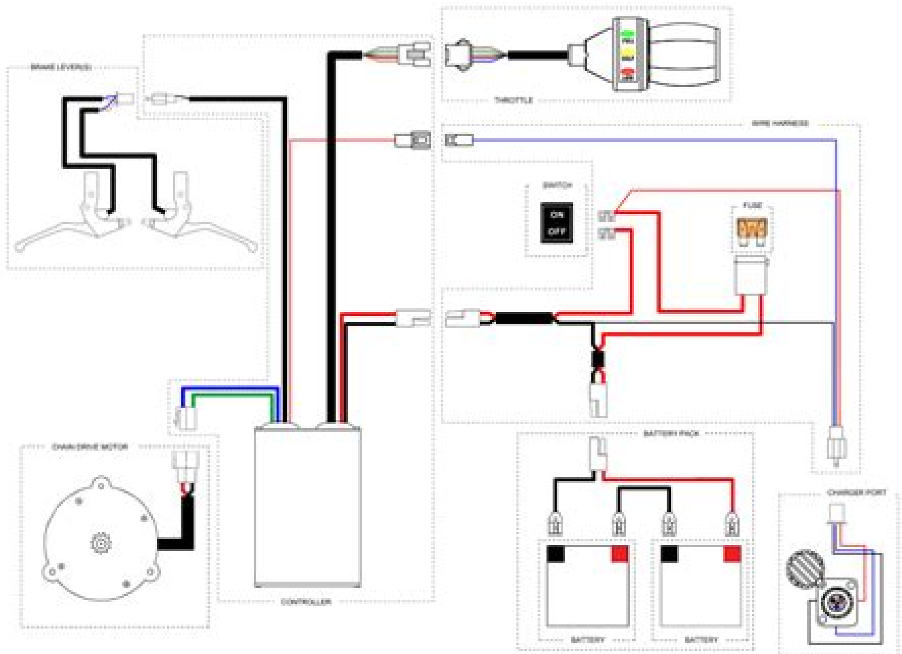
eZip and IZIP 24 Volt Electric Scooter with 3-Wire Charger Port Wiring Diagram
