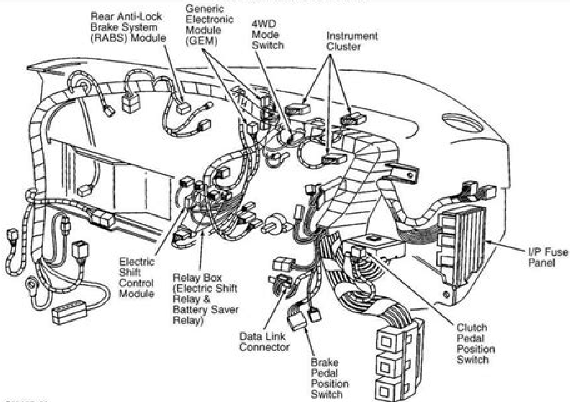
Fig. 2: Locating GEM, Electric Shift Control Module & Relays
