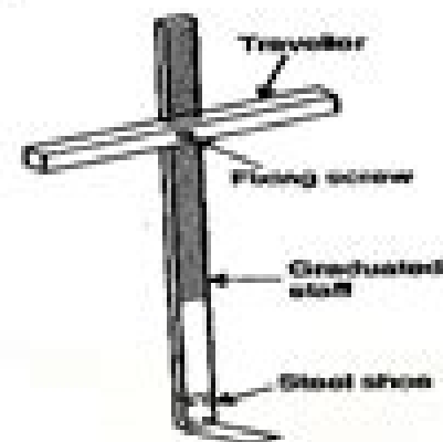
FIG. 20.6. TRAVELLING ROD.
