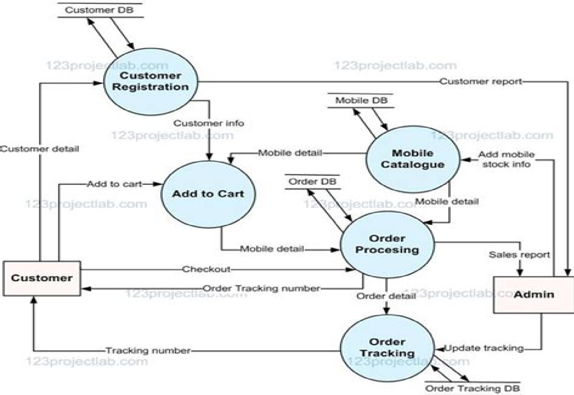
Level-2 DFD for Online Mobile Shop Management System
