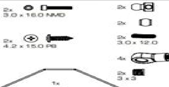
50-020 5512 Anti-roll-bar front Stabi vorne
