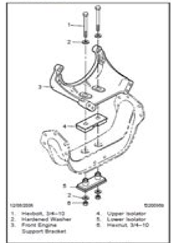
Fig. 2, Front Engine Mounting
