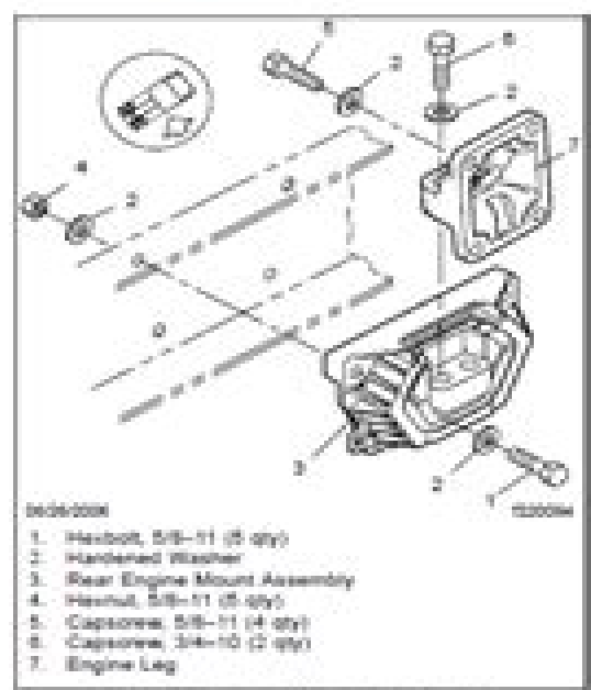
Fig. 1, Rear Engine Mount and Engine Leg
