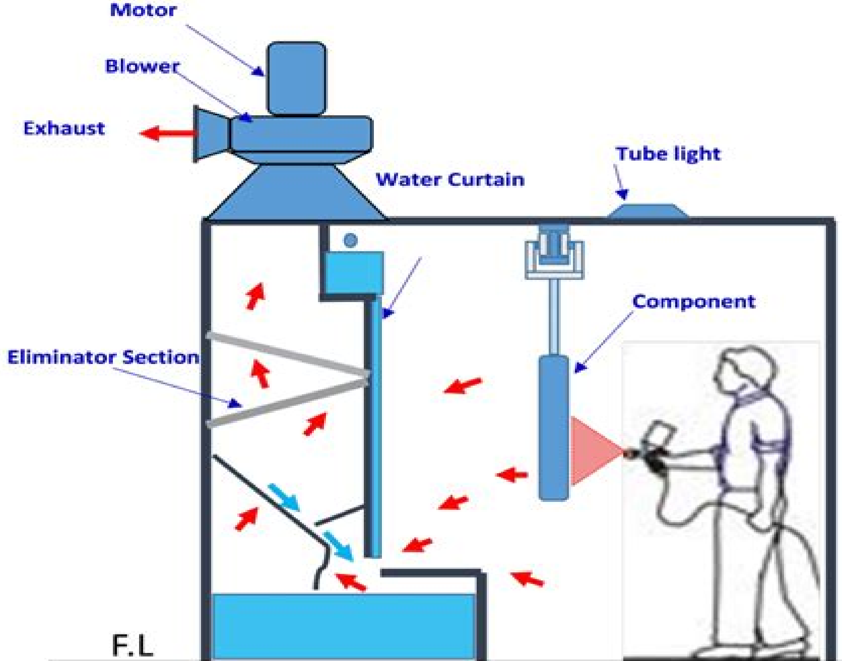
Water Wash Paint Booth
