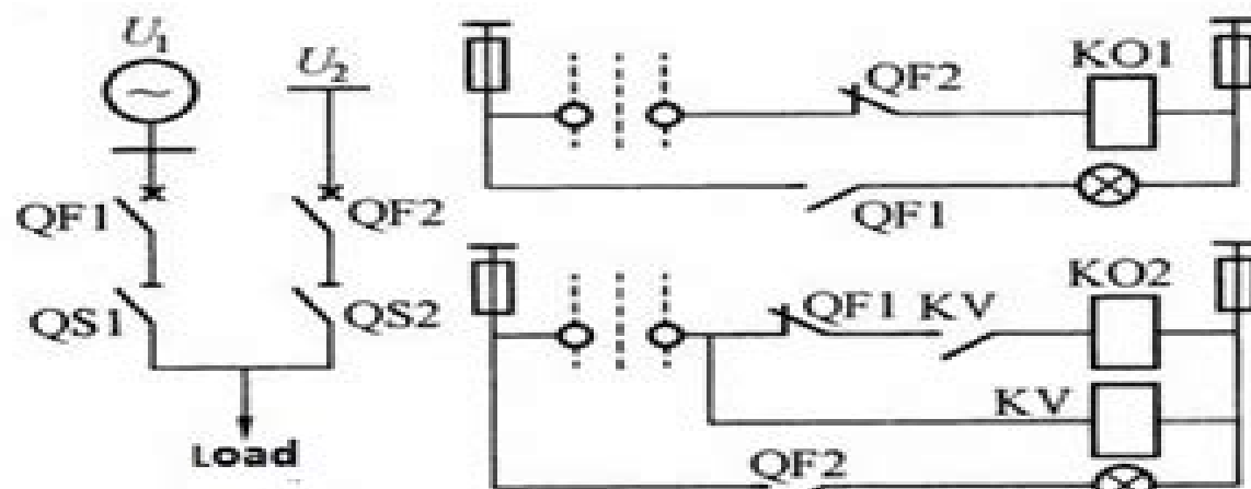
Standby Power supply and external automatic switching Circuit
