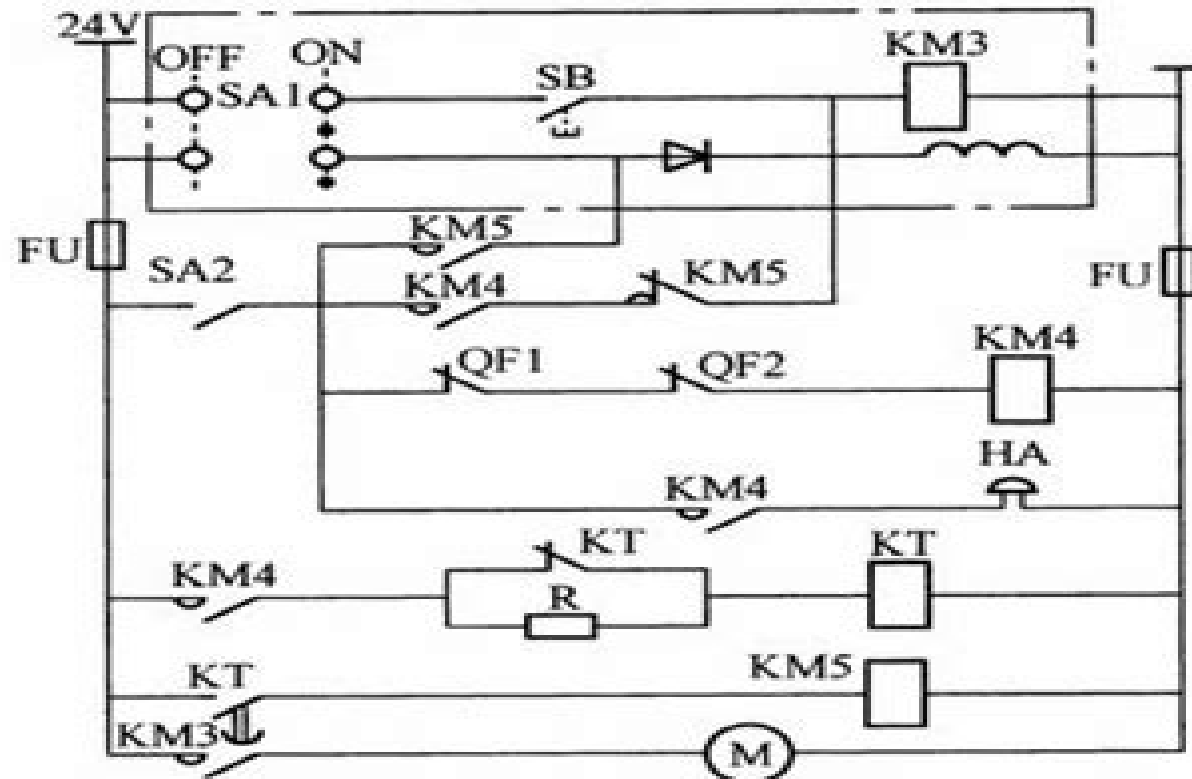
automatic starting device
