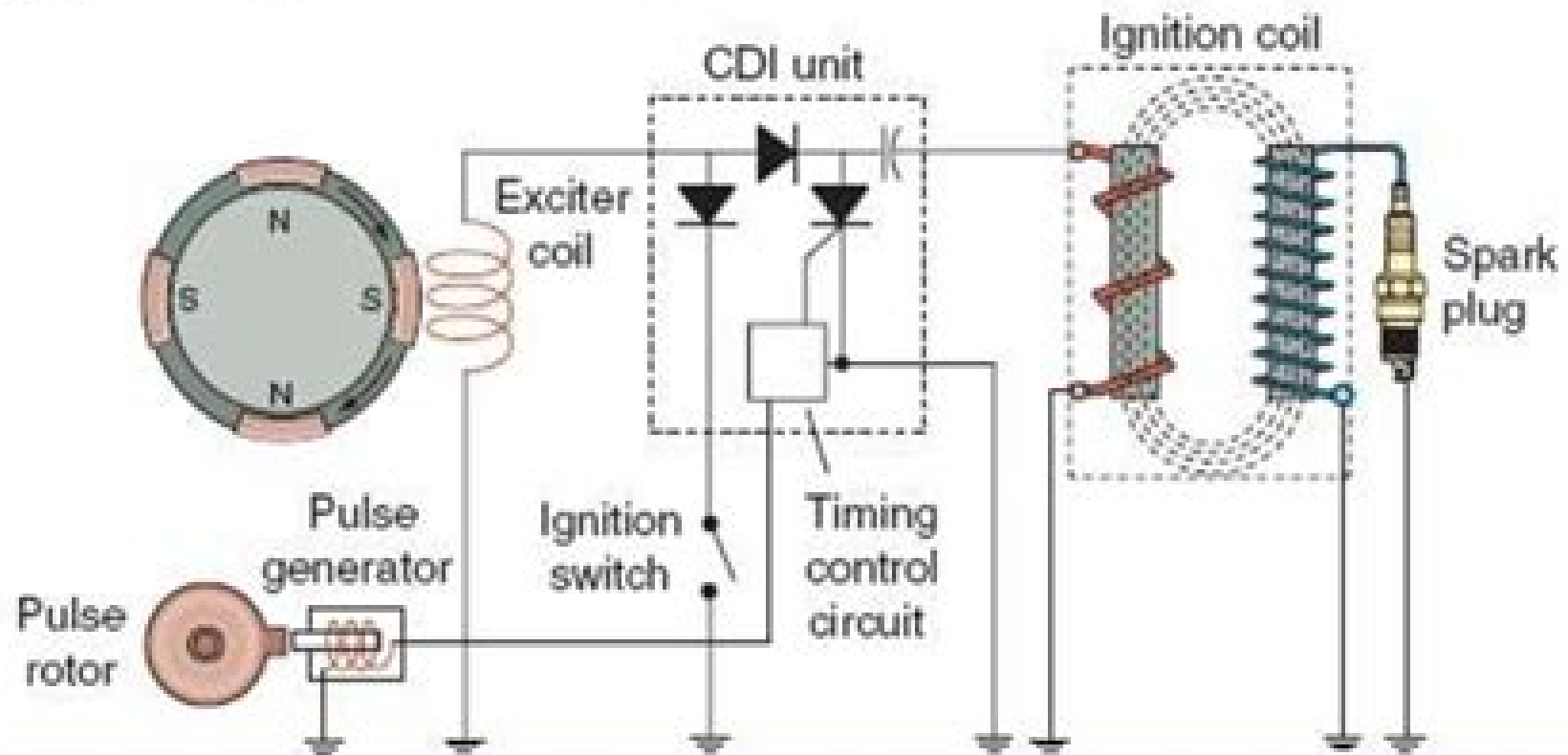
Figure 21 A typical capacitor discharge ignition (CDI) system.
