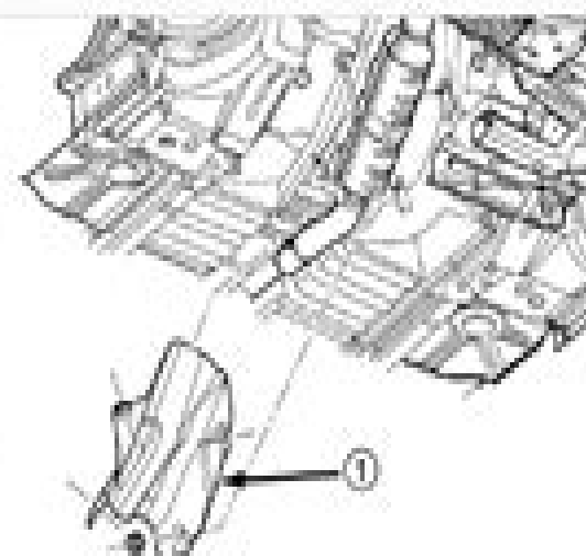
Fig. 152 Converter Heat Shield Removal/Installation 1 - CONVERTER HEAT SHIELD
