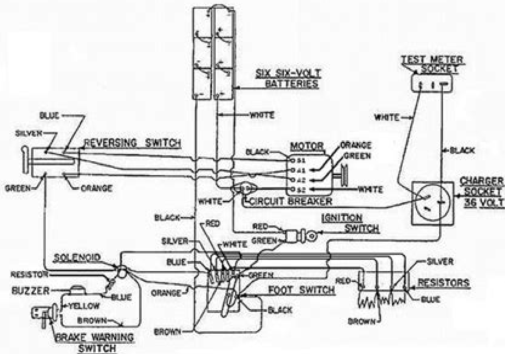
Cushman Wiring Diagram For 36 Volt Model 732
