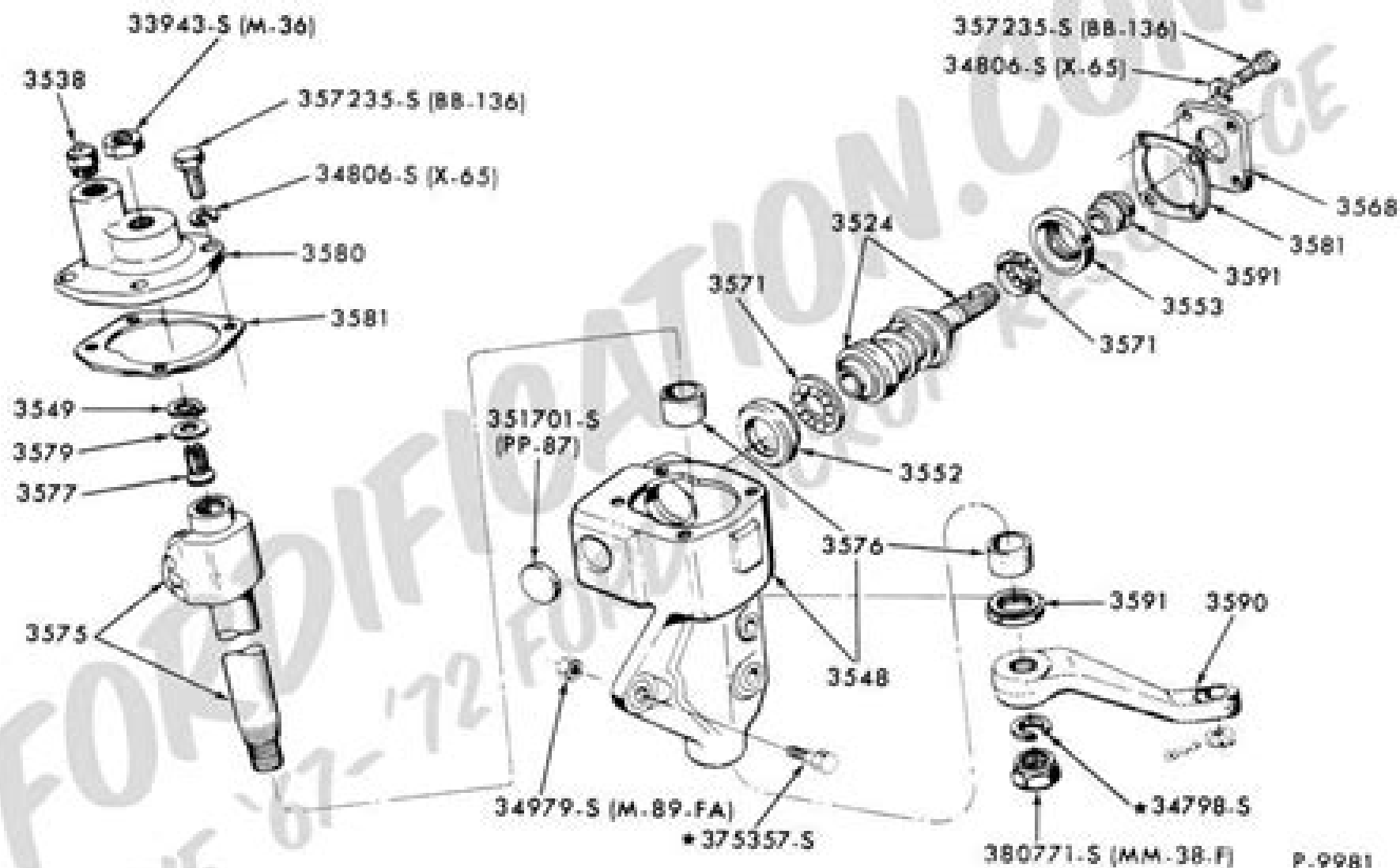
GEAR ASSY. DETAILS-ROSS MODEL 24J 1966/72 F100 (4 x 4)
