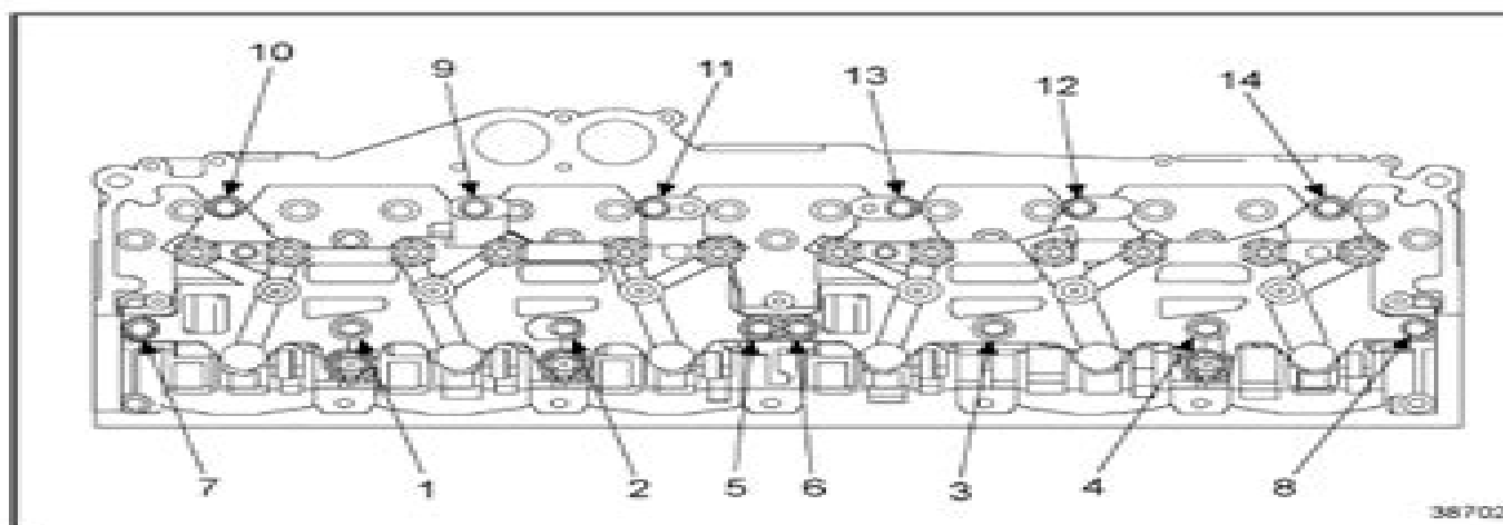
Figure 1-523 Housing Hold-Down Bolt Locations
