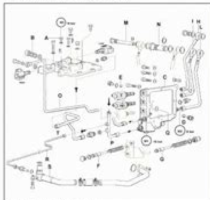
Fig. 36 - Exploded view control unit for Powershift system A - Test fitting for testing pressure (P.T.O. clutch hydraulic circuit) B - Solenoid valve C - Valve body D - Solenoid valve E - Solenoid valve F - Oil pressure regulator valve G - Lubrication pressure control valve H - Solenoid valve I - Solenoid valve J - Solenoid valve K - Solenoid valve L - P.T.O. valve M - P.T.O. valve N - P.T.O. valve O - P.T.O. valve P - P.T.O. valve Q - P.T.O. valve R - P.T.O. valve S - P.T.O. valve T - P.T.O. valve 1 - Solenoid valve 2 - Solenoid valve 3 - Solenoid valve 4 - Solenoid valve 5 - Solenoid valve 6 - Solenoid valve 7 - Solenoid valve 8 - Solenoid valve 9 - Solenoid valve 10 - Solenoid valve
