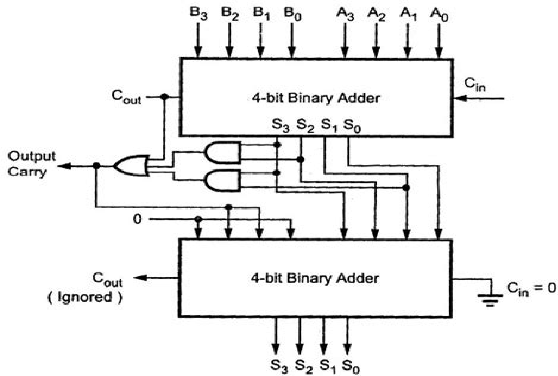
Fig. 3.32 Block diagram of BCD adder
