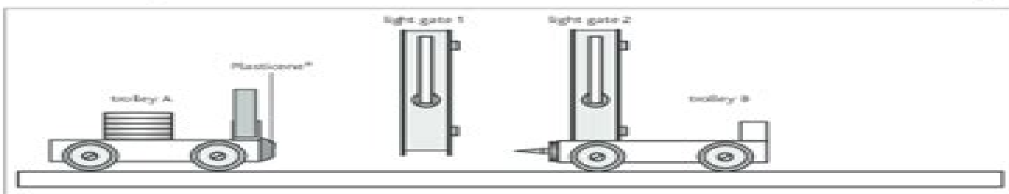
Figure 1: Arrangement of large trolleys to investigate momentum and momentum conservation
