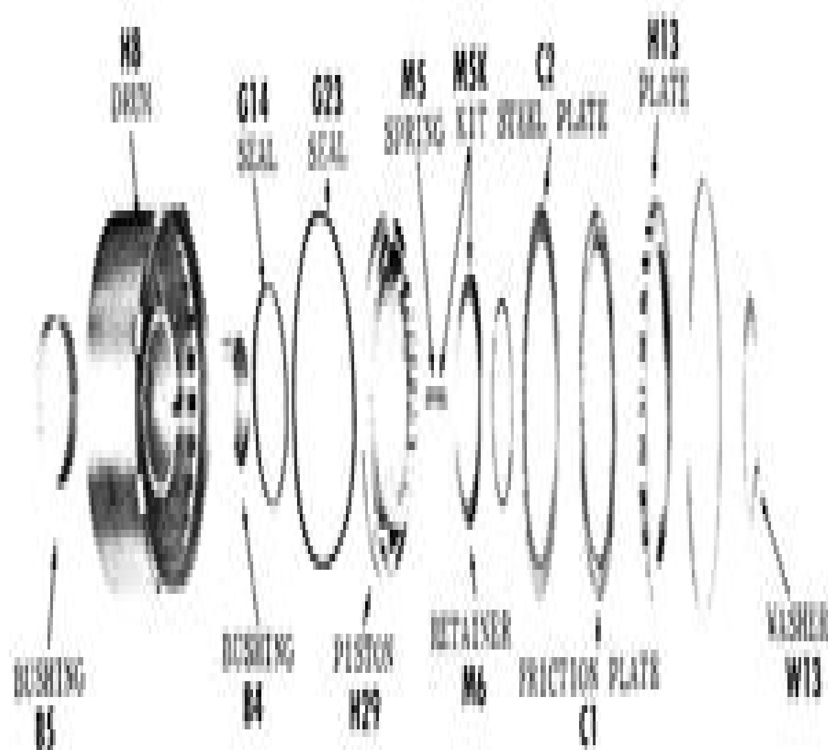
DIRECT DRIVE CLUTCH
