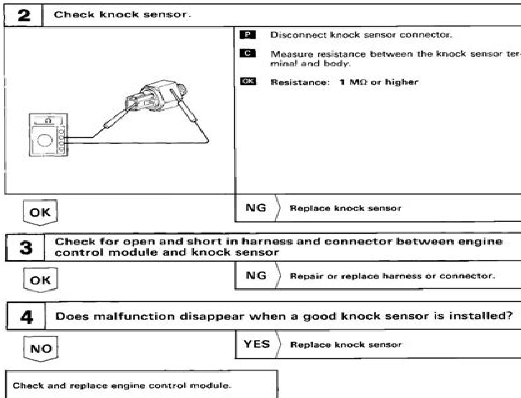
Fig. 58: DTC 52 - Diagnostic Flowchart (1 Of 2) Courtesy of TOYOTA MOTOR SALES, U.S.A., INC.
