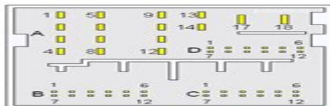
52 pin Volkswagen Quadlock connector
