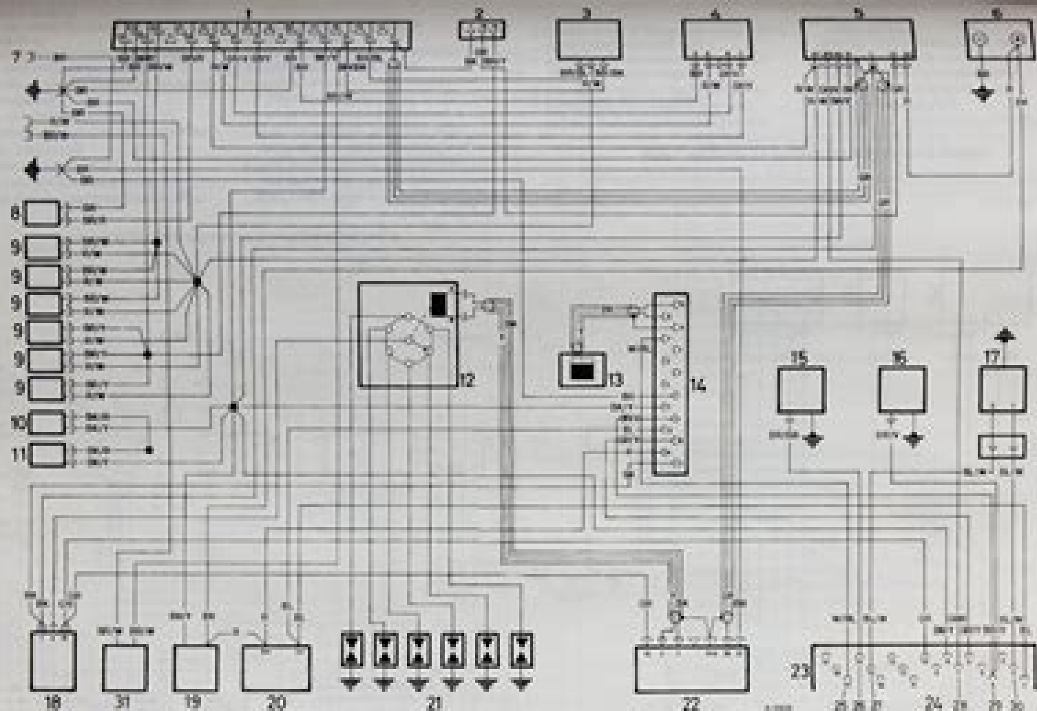
Key to wiring diagram for Series 2 engine electronics and fuel injection
