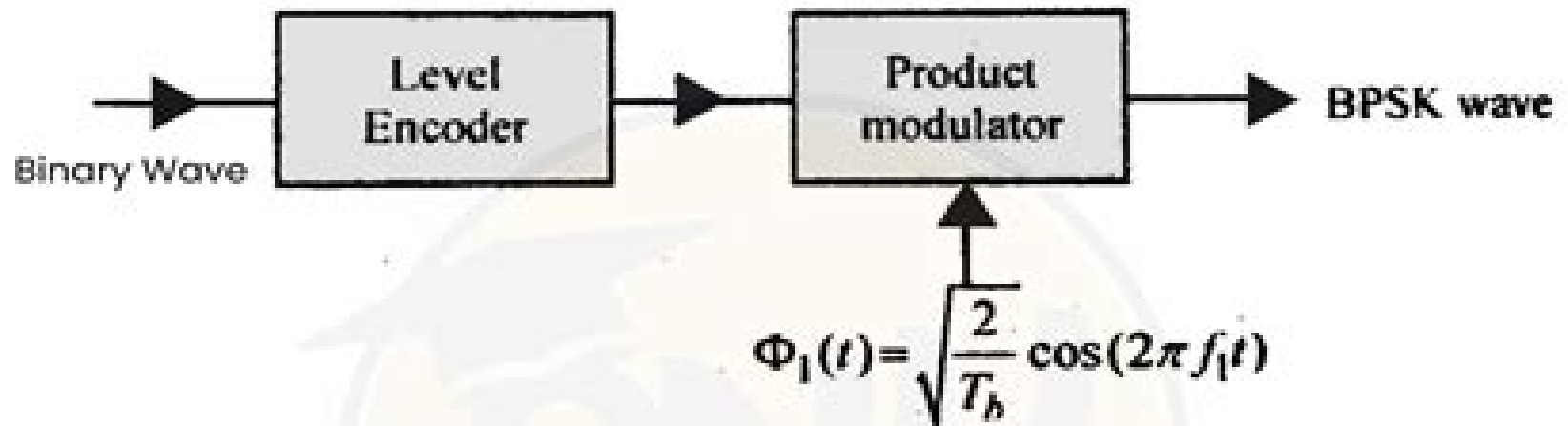
Block Diagram of BPSK Transmitter
