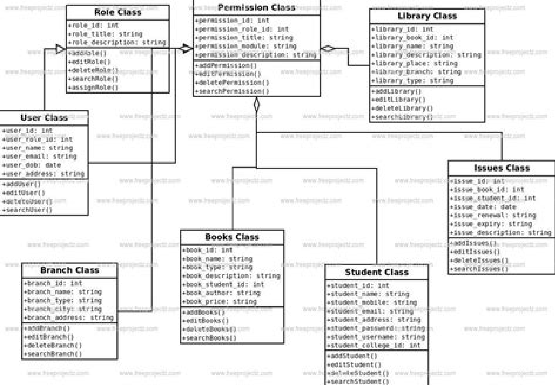
Class Diagram of College Management System
