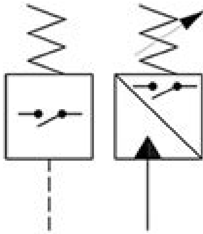
Pressure Switches
