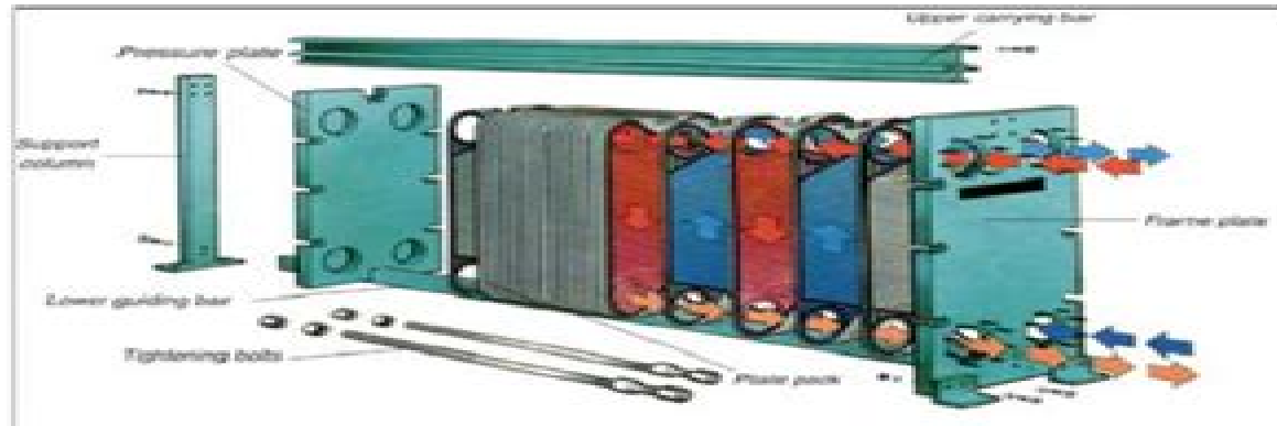
Figure 2-14: Plate Heat Exchanger
