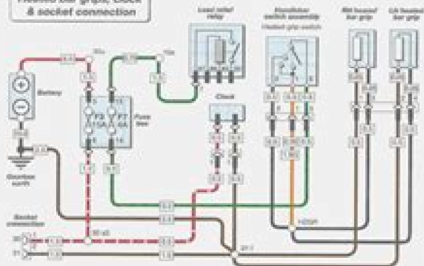
R850 R (2003-on) and R1150 R : Heated bar grips, clock and socket connection
