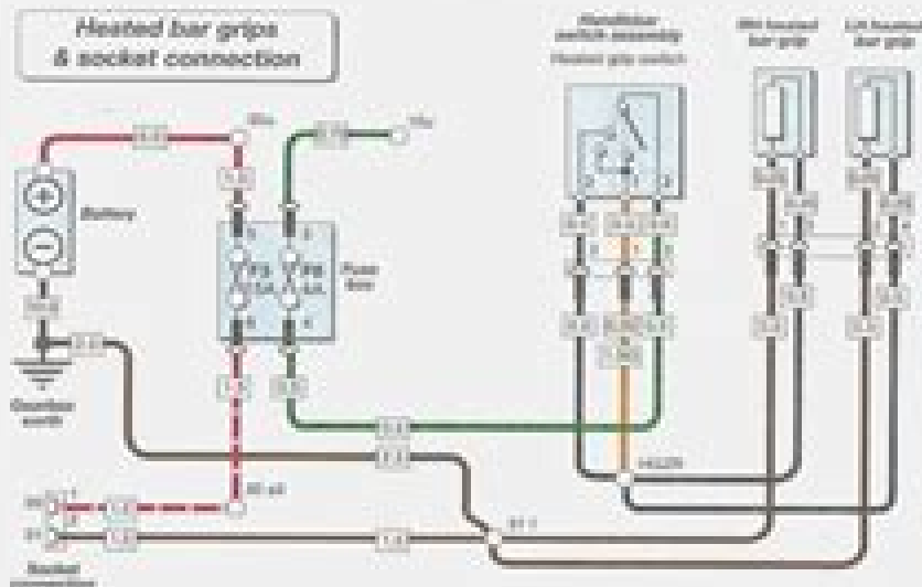
R1100 S ('99 and '00) Heated bar grips and socket connection
