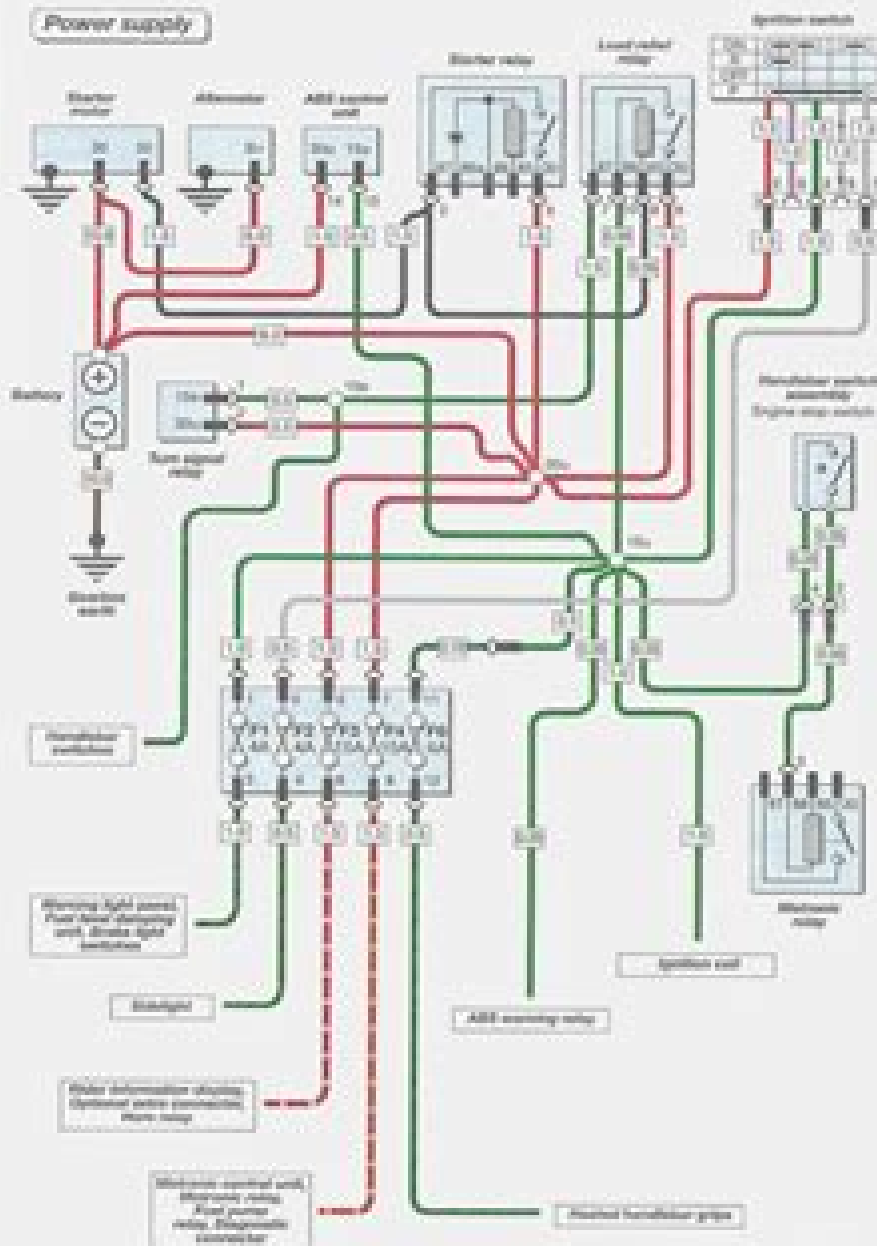
R1100 S ('99 and '00) : Power supply
