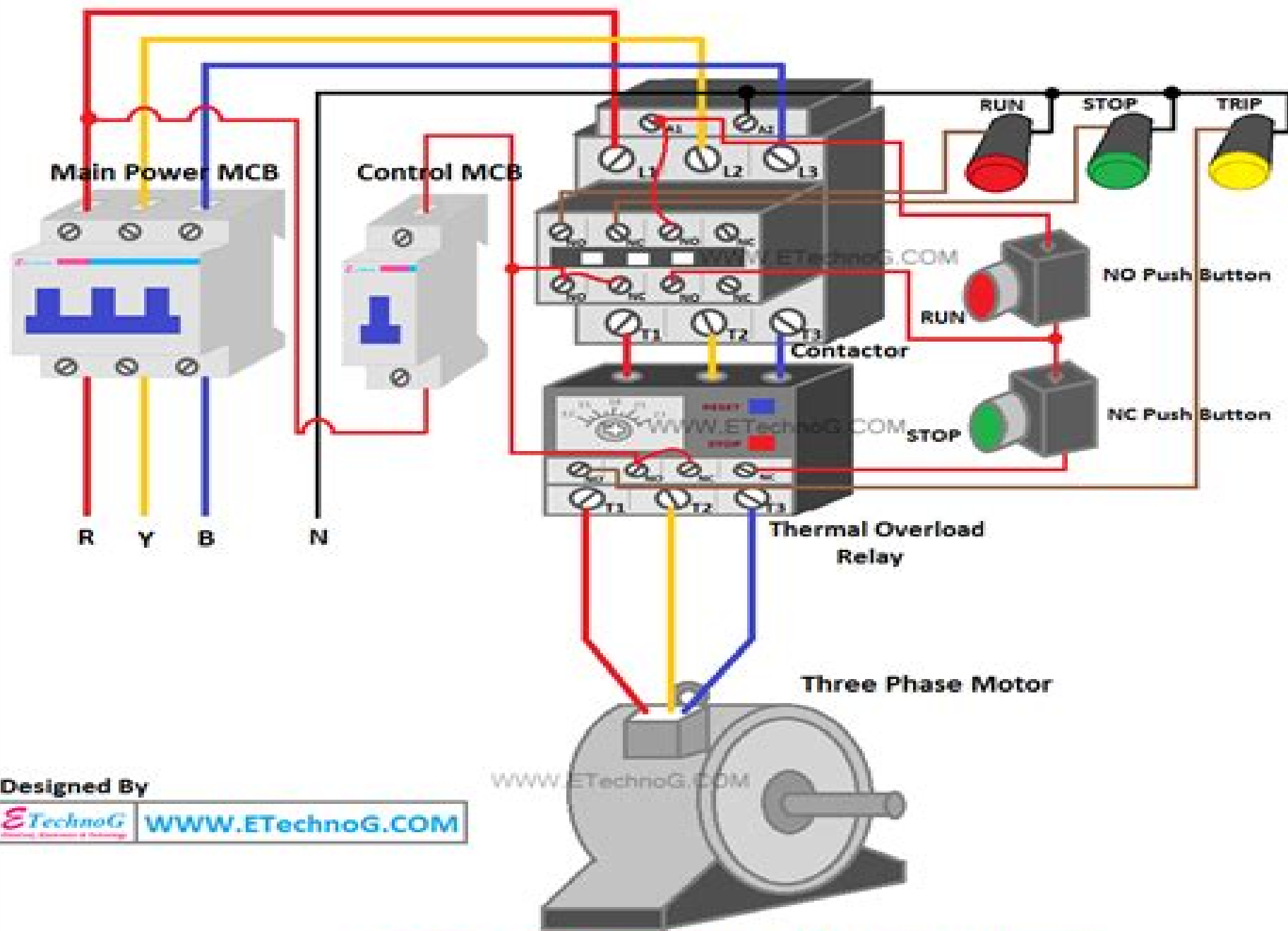
DOL Starter Connection & Wiring Diagram
