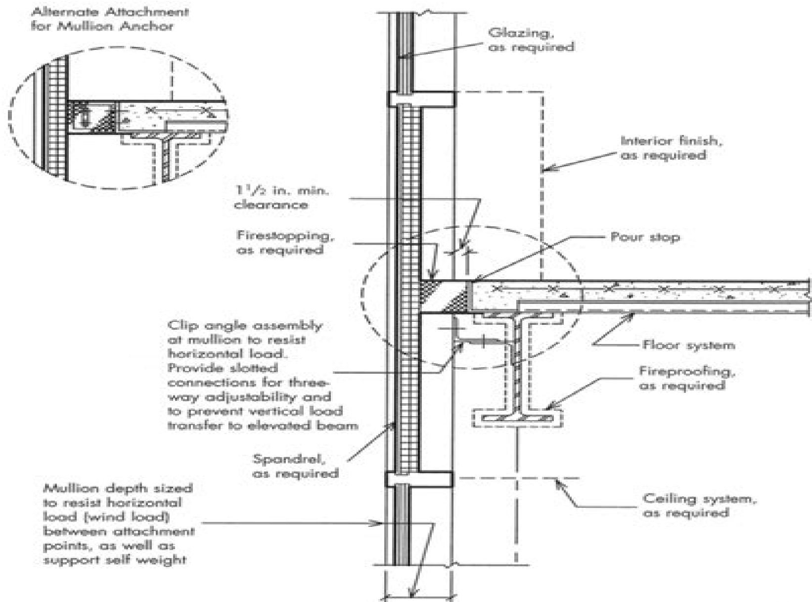
Fig. 4. Sample wall section detail for curtain wall enclosure systems.
