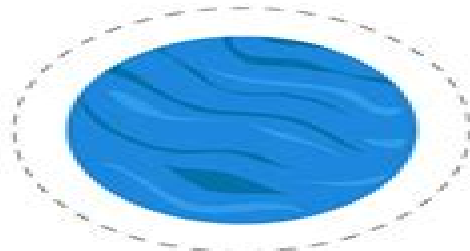
Neptune
