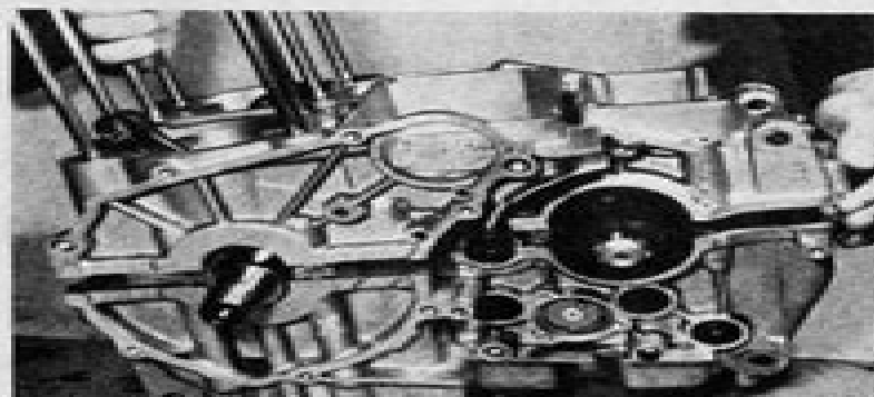
35.2 Lower upper casing into place over gearshafts and crankshaft
