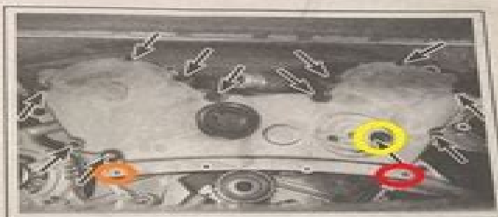
6.6b Location of the upper timing belt mounting fasteners
