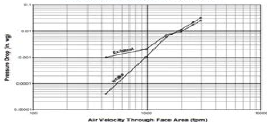
PRESSURE DROP GRAPH - 36" x 36"
