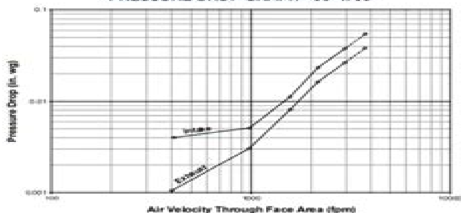
PRESSURE DROP GRAPH - 36" x 36"
