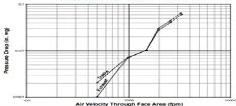
PRESSURE DROP GRAPH - 24" x 24"
