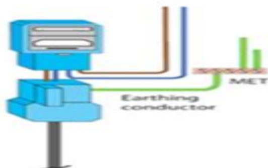
TN-C-S System
