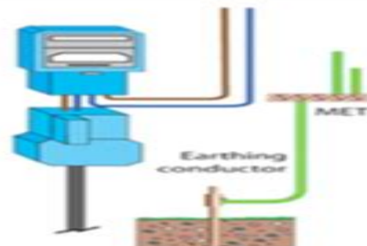
TT System
