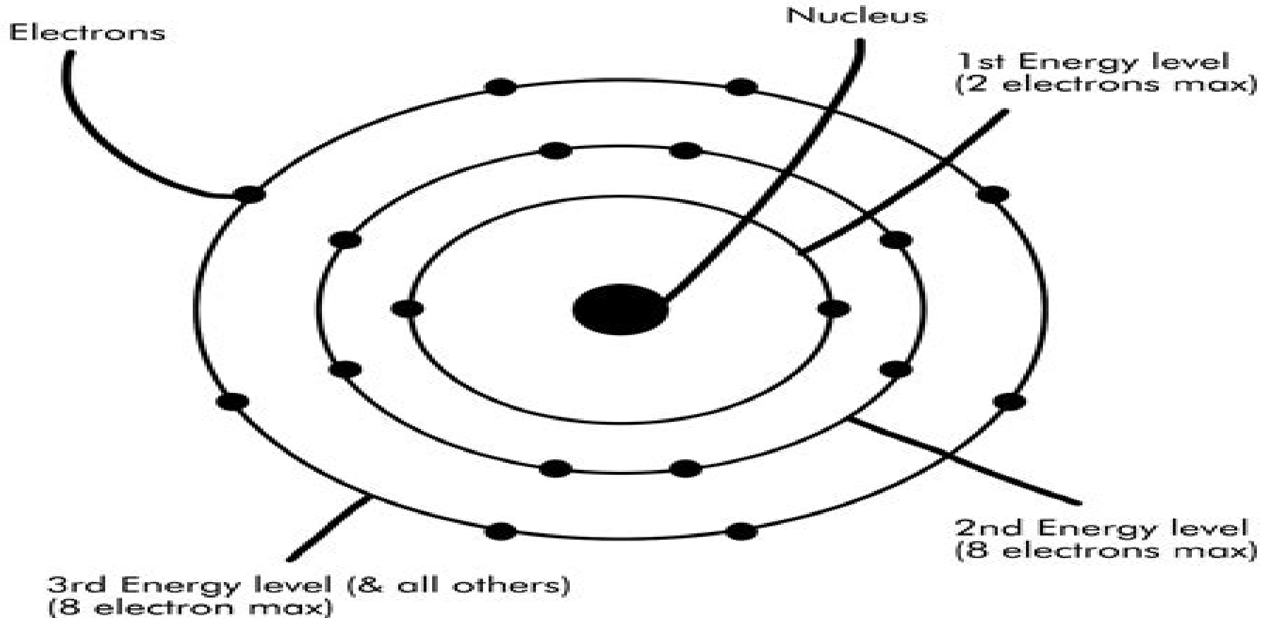
Electron Energy Levels
