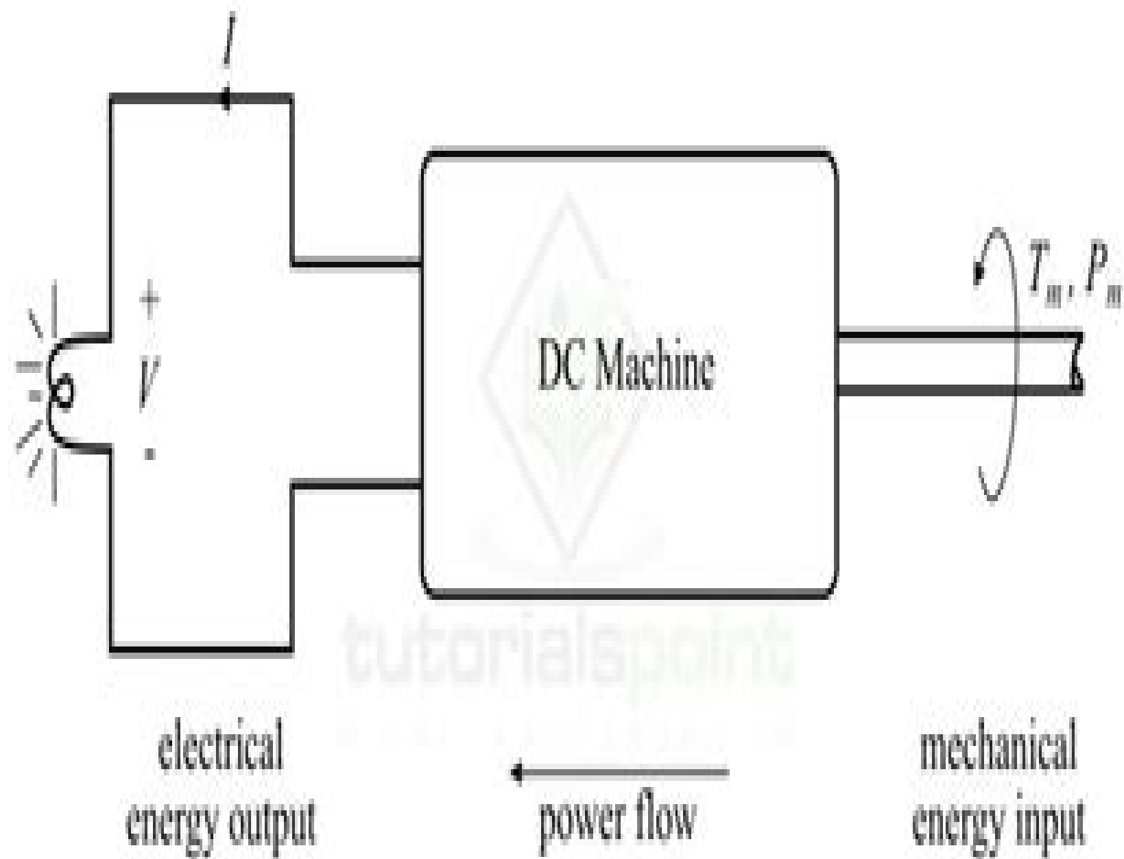
Figure 2 - DC Machine as Generator
